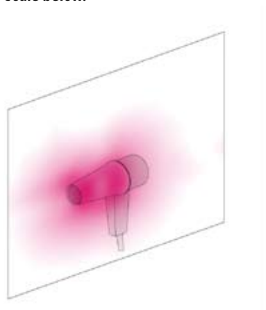
Magnetic field of a hairdryer. The most intensive fields occur close to the casing. The significance of the solid lines is indicated in the colour scale below.
